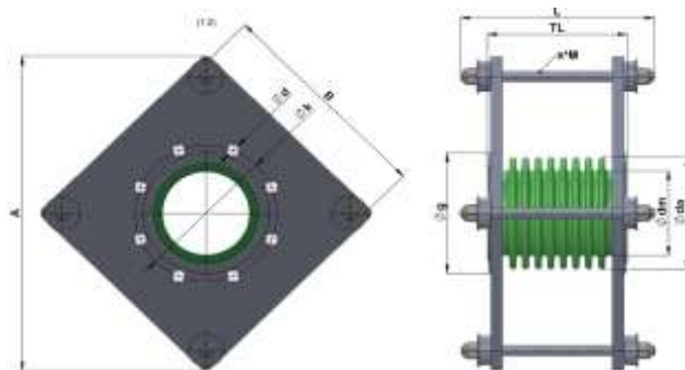
Fig. 3: Square flange
