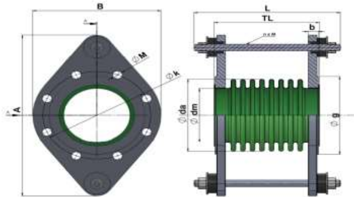
Fig. 1: Oval flange
