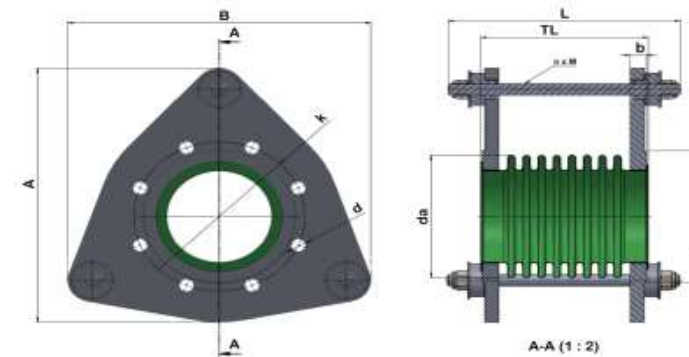
Fig. 2: Triangular flange
