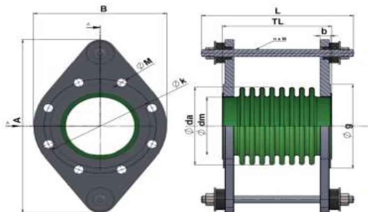
Fig. 1: Bride ovale
